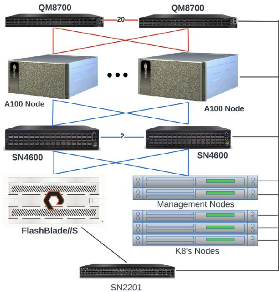
FIGURE 2 AIRI Network connectivity overview
