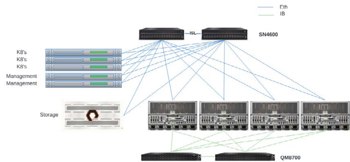
FIGURE 12 Logical topology for a four-node AIRI system with NVIDIA Quantum InfiniBand compute fabric
